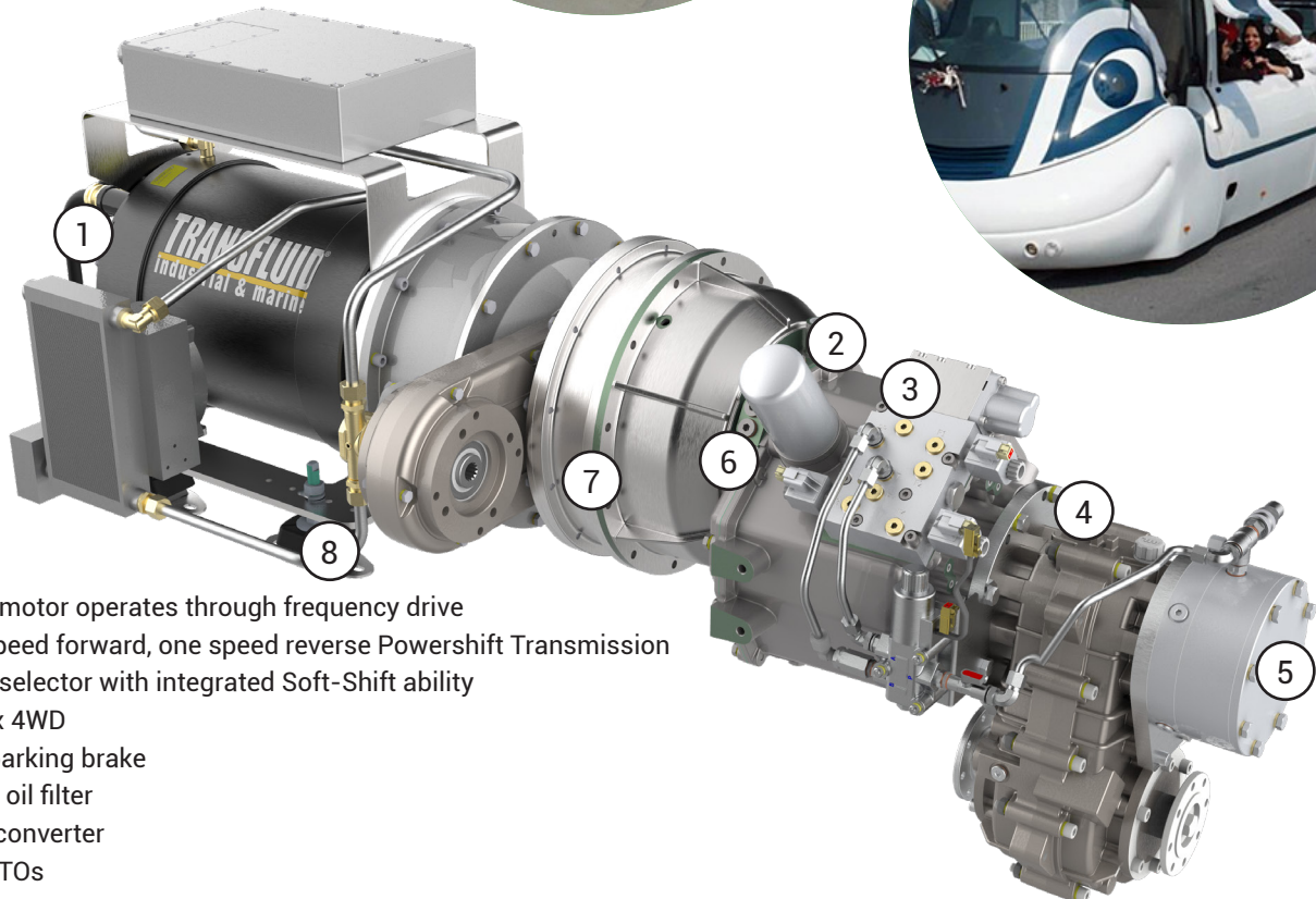
[Example of full power-train supply]
